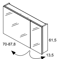
Camerino 70 2P BINOVA-NIKA F-13,5 / BINOVA-NIKA cupboard 70 2D D-13,5
