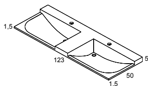
Lavabo 123 acrílico OPEN F-50 / OPEN acrylic washbasin 123 D-50
